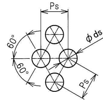
SCREEN DETAIL
