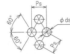
ST'D SCREEN DETAIL
