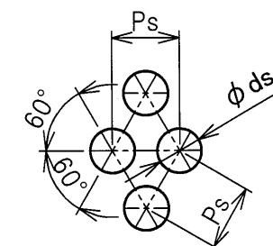
STANDARD SCREEN DETAIL
