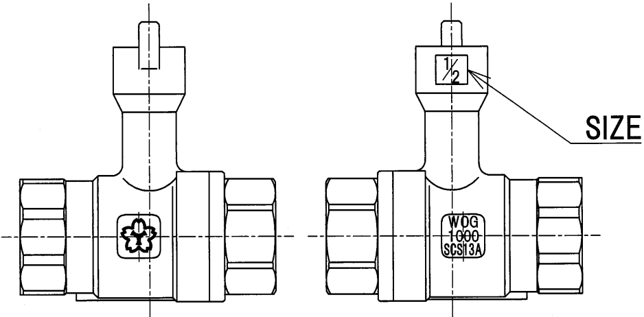
MARKING (SIZE 15)
